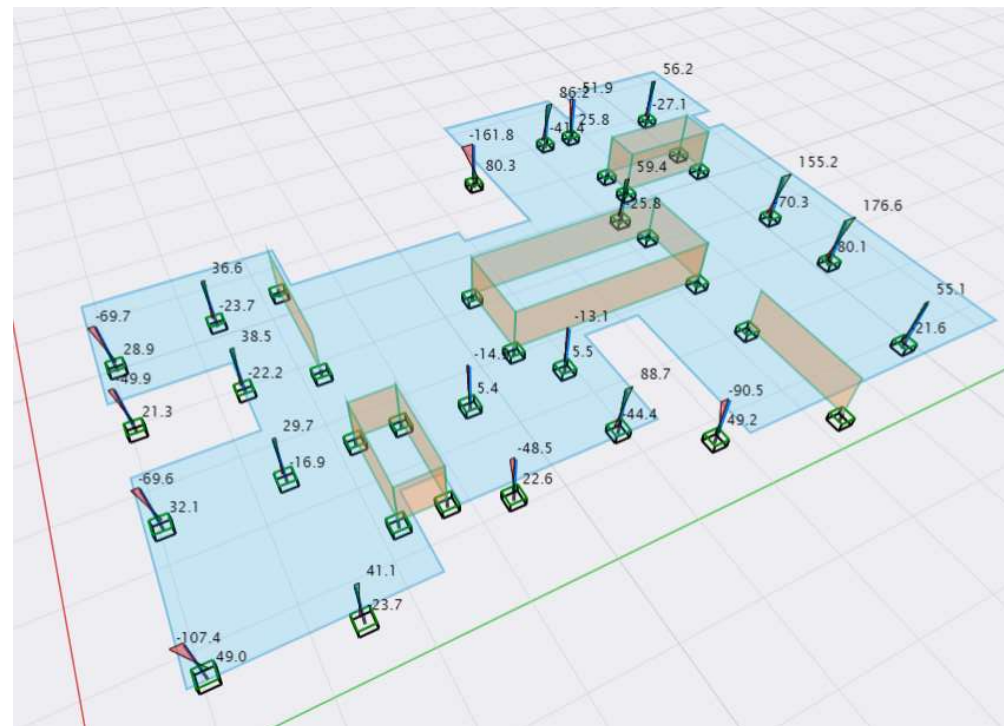
M33 Force Diagram (Frames)
