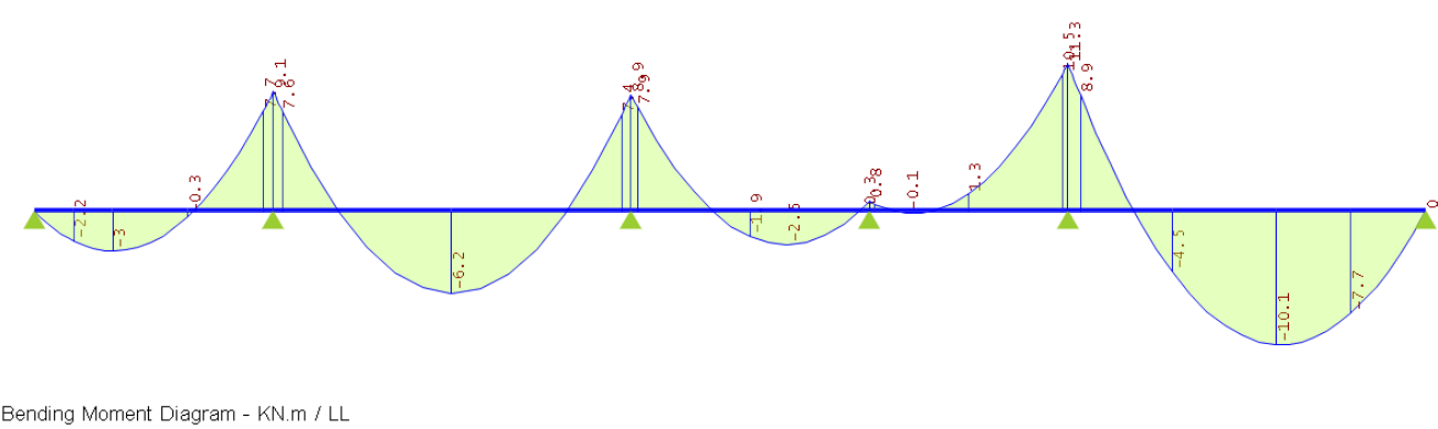
Bending Moment Diagram - KN.m / LL
