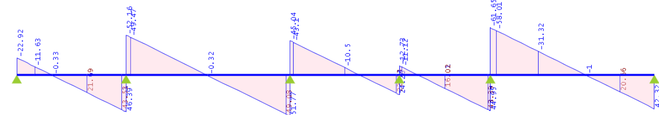
Shear Force Diagram - KN , m / LC-1.2DL+1.5LL
