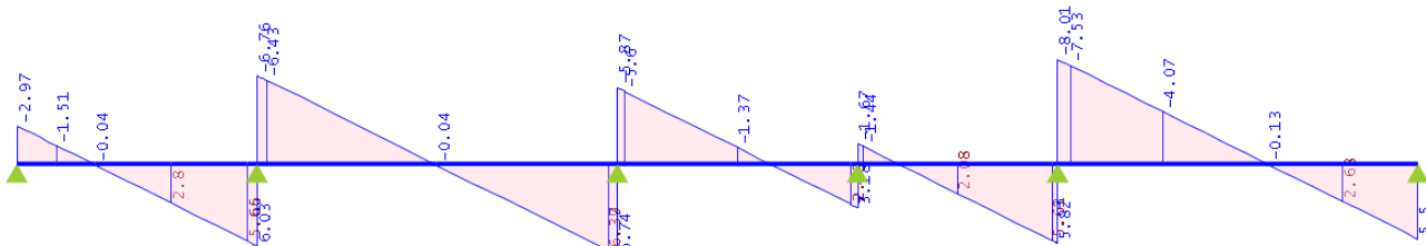
Shear Force Diagram - KN , m / SDL
