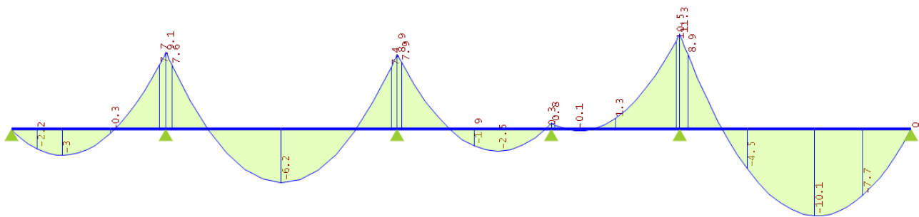
Bending Moment Diagram - KN.m / SDL
