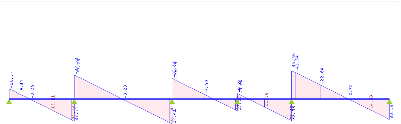
Shear Force Diagram - KN , m / LC-1.0DL+0.4LL+PT
